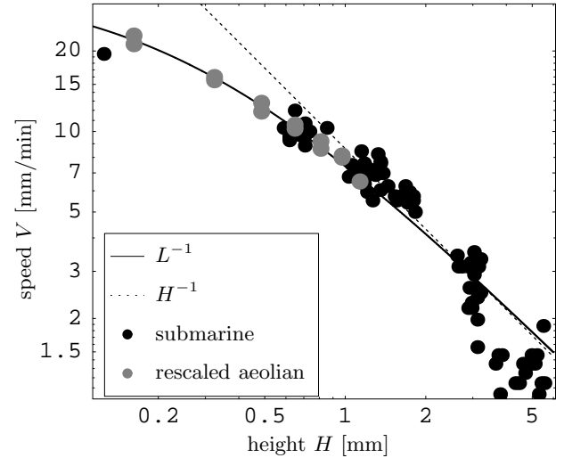
FIG. 1: Submarine (black [1]) and aeolian (gray [4]; rescaled) migration speed data compared to H^{-1} (dotted [1]) failing for small dunes, and L^{-1} (solid [3]) compatible with the data.
